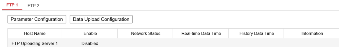
Figure 11-2 Custom Settings
