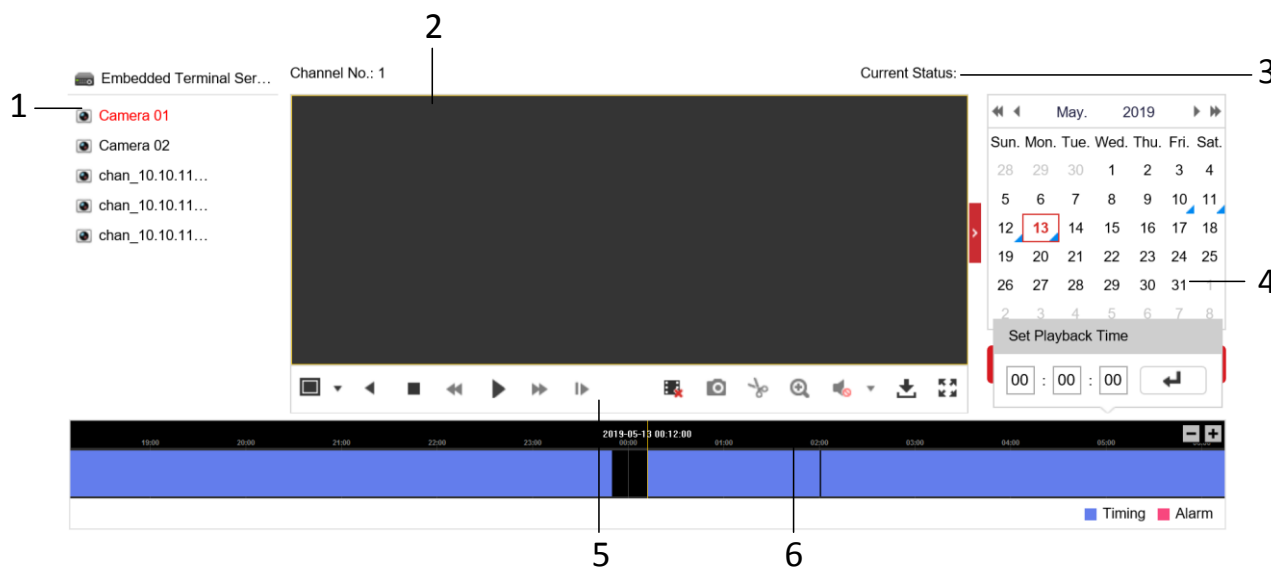
Figure 4-3 Playback Interface
