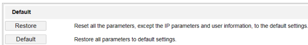
Figure 14-4 Default
