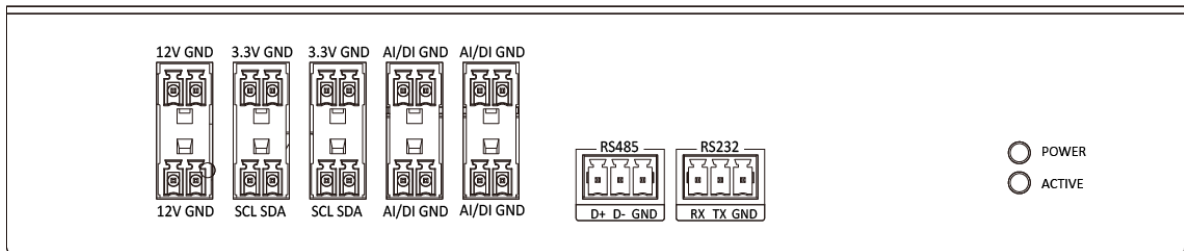
Figure 1-1 Front Panel
