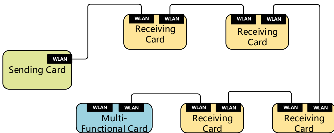
Figure 2-1 Hardware Connection
